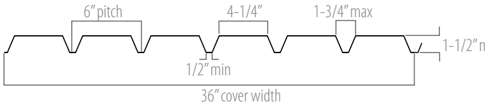
F DECK (INTERMEDIATE RIB)
