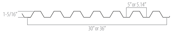
EXTRA HEAVY DUTY (TF125, 1.3C, EHD, UFX, CF 1 3/8)
