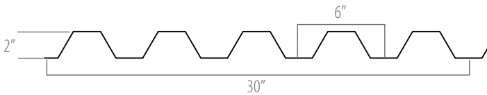
SUPER DUTY (TF200, 2C, UF2X, E200)
