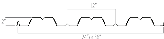
2" COMPOSITE FLOOR DECK (SB200, 3VLI, CFD2, 2" LOK FLOOR, 2.0 CF, 2.0CD)
