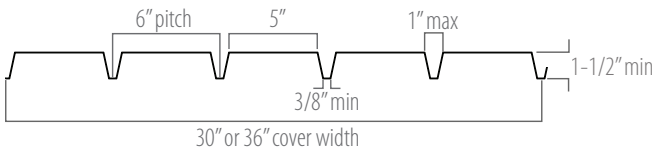
A DECK (NARROW RIB)
