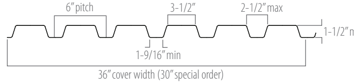
B DECK (WIDE RIB)
