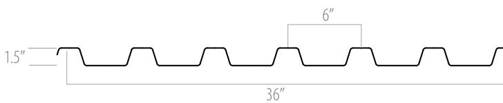
1.5" INVERTED (TF150, 1.5C, ISD, EF, 1.5 FD)
