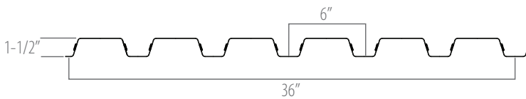
1.5" COMPOSITE FLOOR DECK (SB150, 1.5VL, CFD 1.5, B-LOK, 1.5CF, EC 150, 1.5CD)
