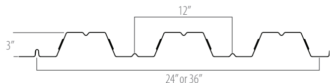
3" COMPOSITE FLOOR DECK (SB300, 3VLI, CFD3, 3" LOK FLOOR, 3.0 CF, 3.0CD)
