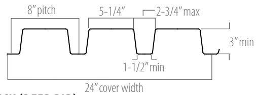
N DECK (DEEP RIB)
