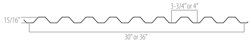
HEAVY DUTY (TF75, 1.0C, HD, UFIX, HF, CF 7/8, 1.0 FD)
