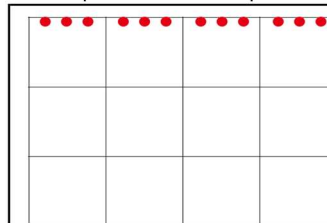
Fasteners @ perimeter supports parallel to deck span
